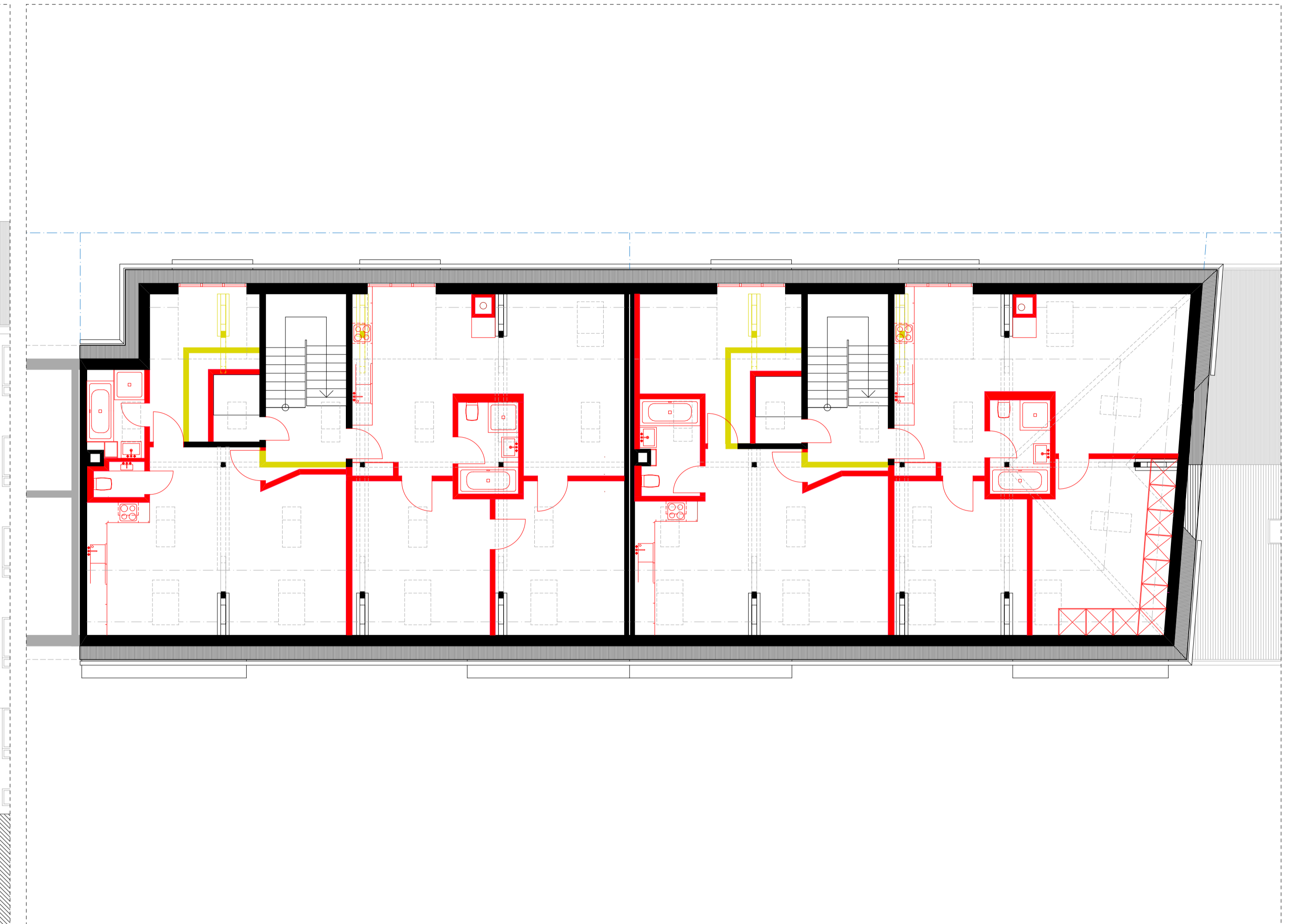
B_001 5. DECKENSCHESS 1:100
